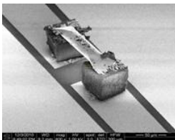
SEM micrographs of test vehicle for vertical interconnects
